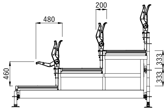
Modulo base. (misure in mm)
